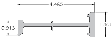
ES-8000T-011 STIFFNER MULLION DOOR
