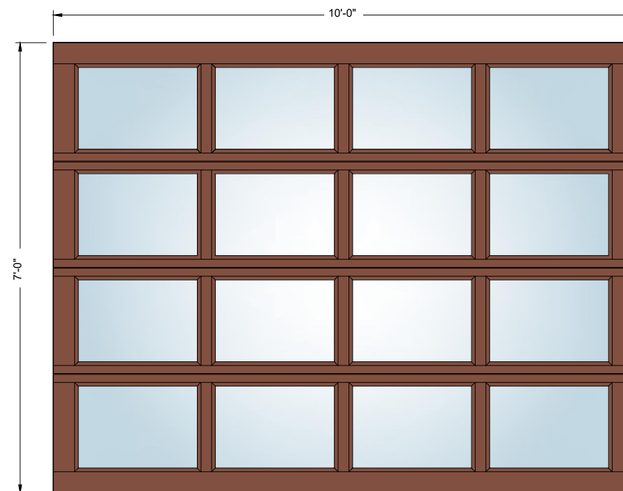
10' x 7' 4-Lite
