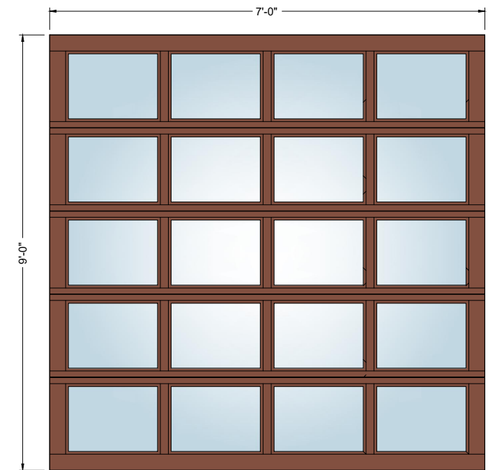
7' x 9' 4-Lite
