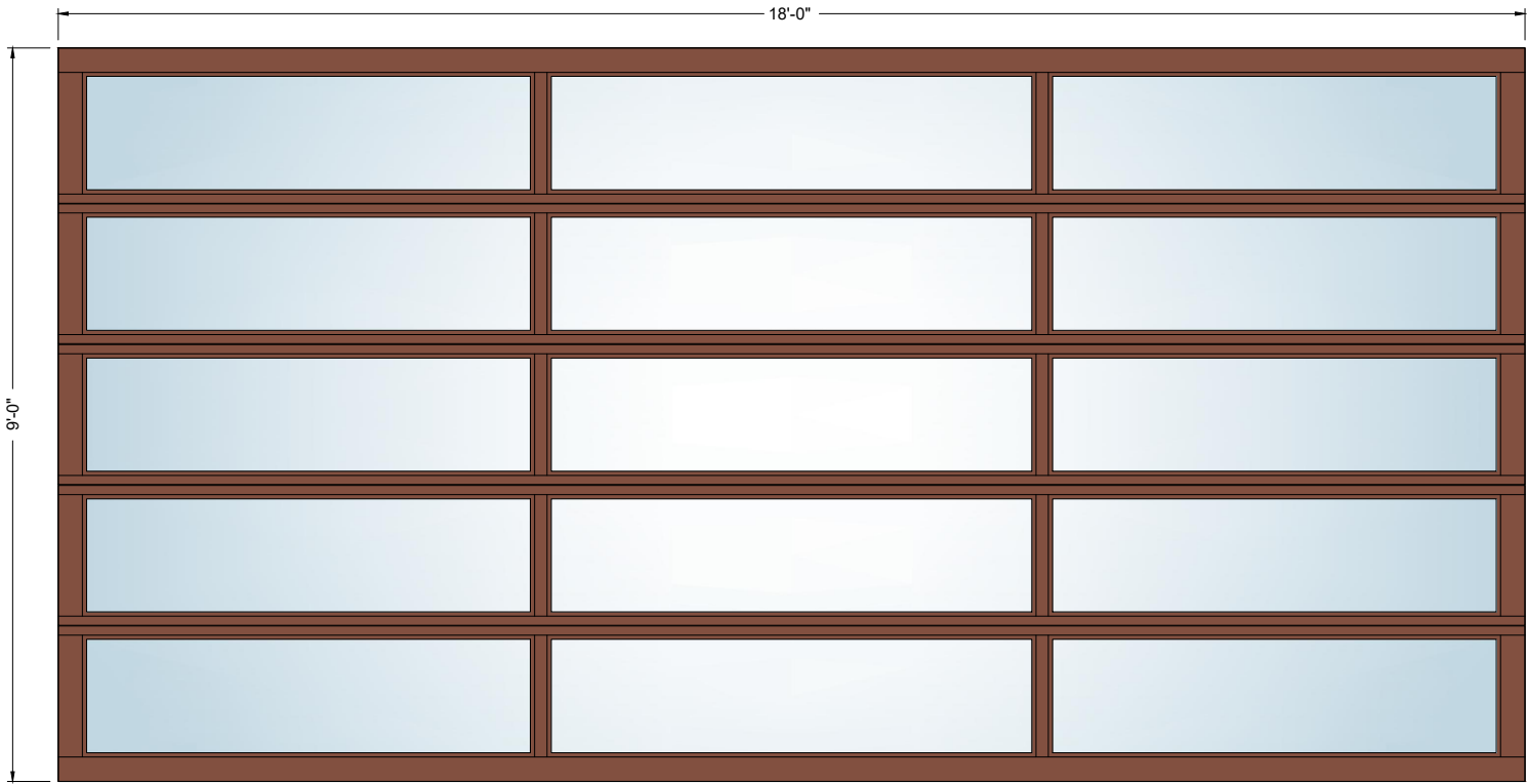
18' x 9' 3-Lite * Low-E unavailable in 5/16" glas
