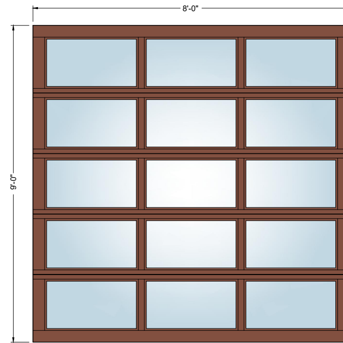
8' x 9' 3-Lite
