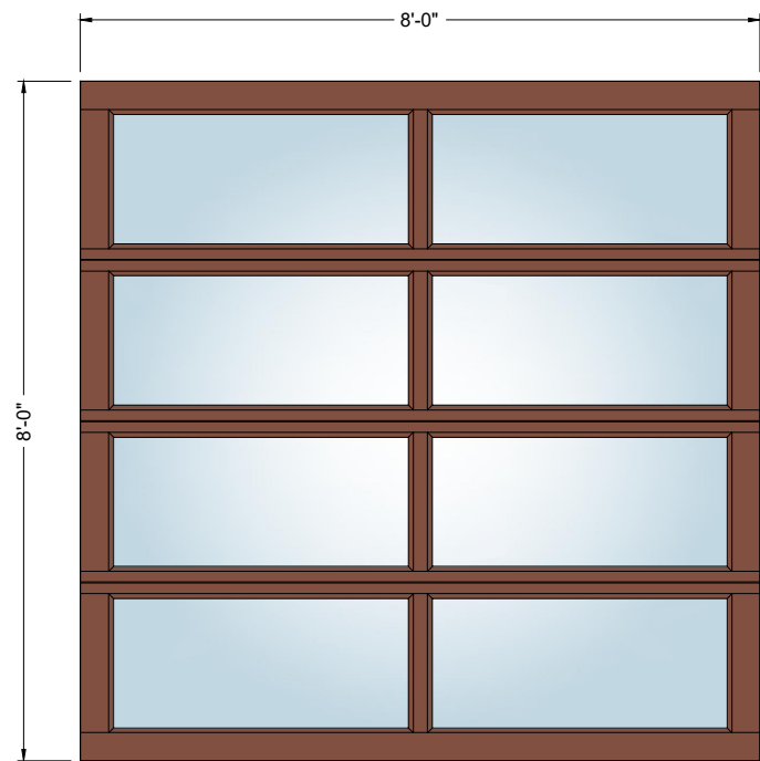
8' x 8' 2-Lite
