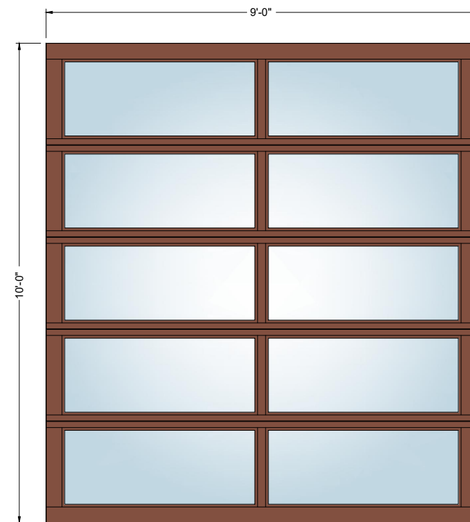
9' x 10' 2-Lite
