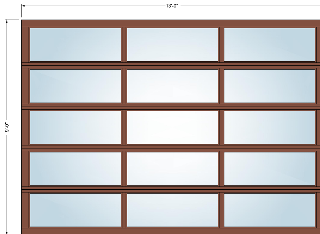
13' x 9' 3-Lite
