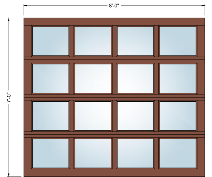
8' x 7' 4-Lite
