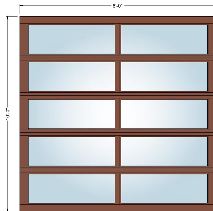
6' x 10' 2-Lite
