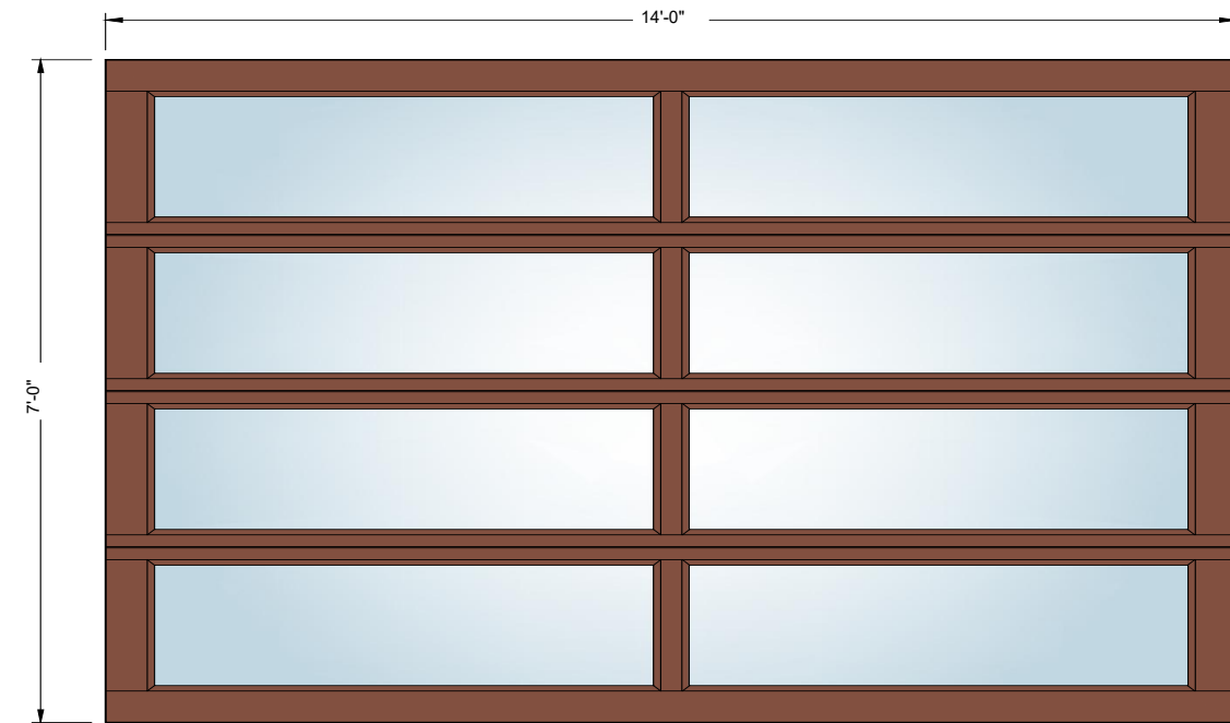
14' x 7' 2-Lite
