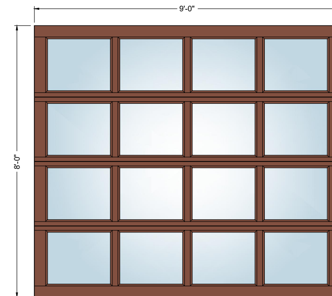
9' x 8' 4-Lite
