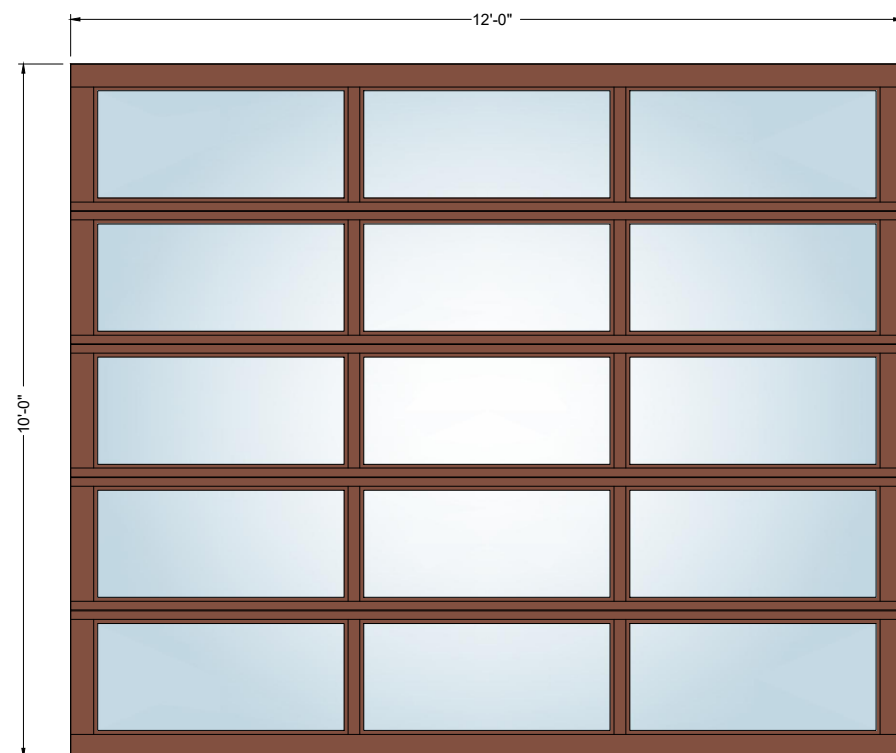
12' x 10' 3-Lite
