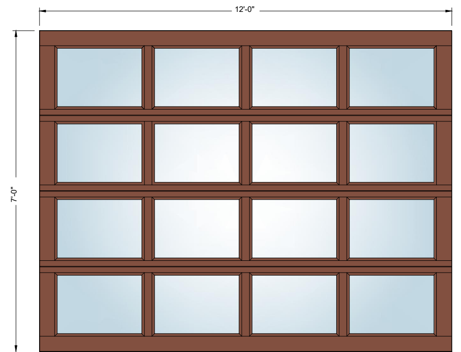
12' x 7' 4-Lite
