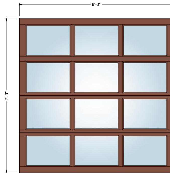
7' x 8' 3-Lite
