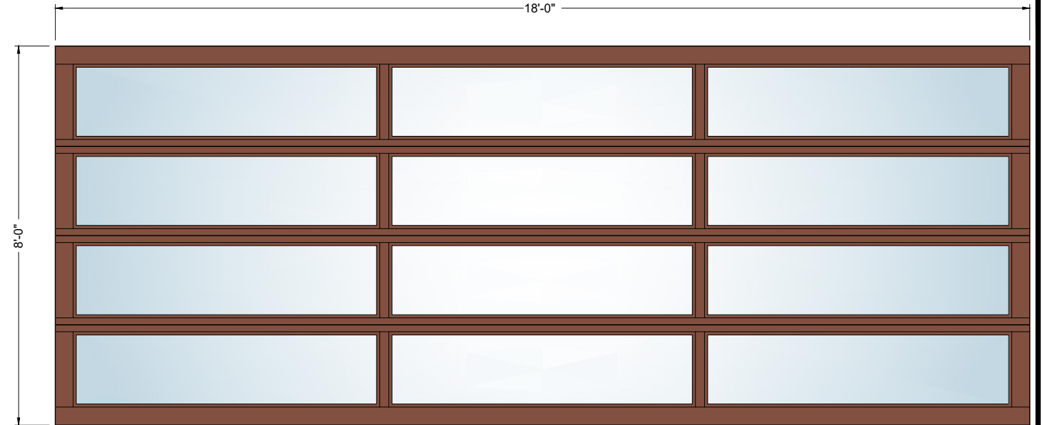
18' x 8' 3-Lite
