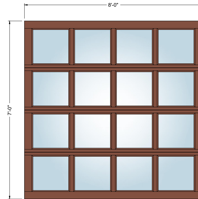
7' x 8' 4-Lite
