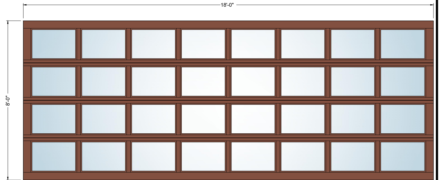
18' x 8' 8-Lite
