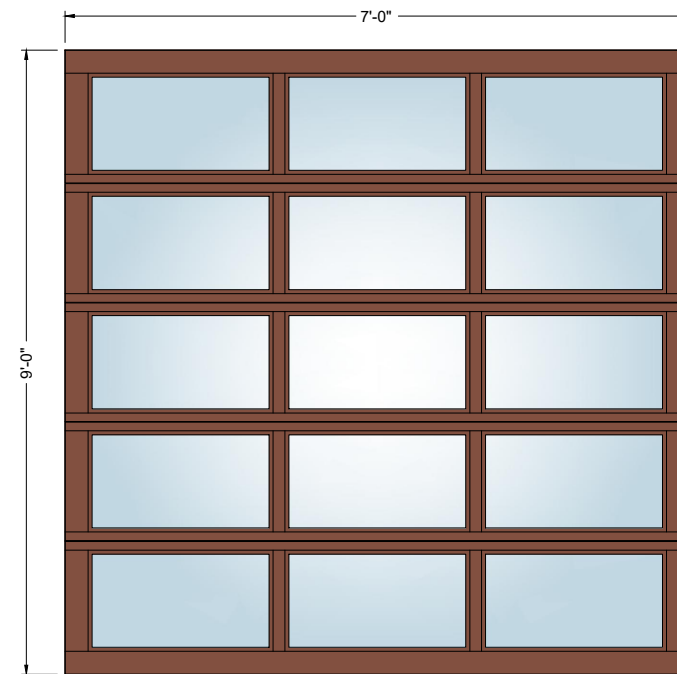
7' x 9' 3-Lite
