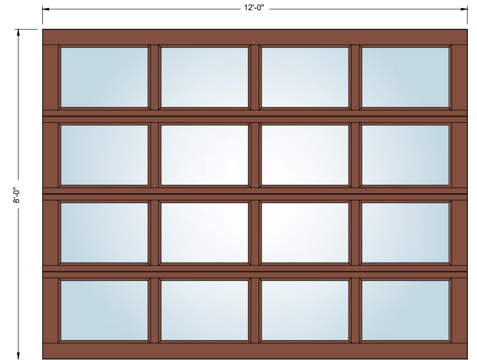
12' x 8' 4-Lite
