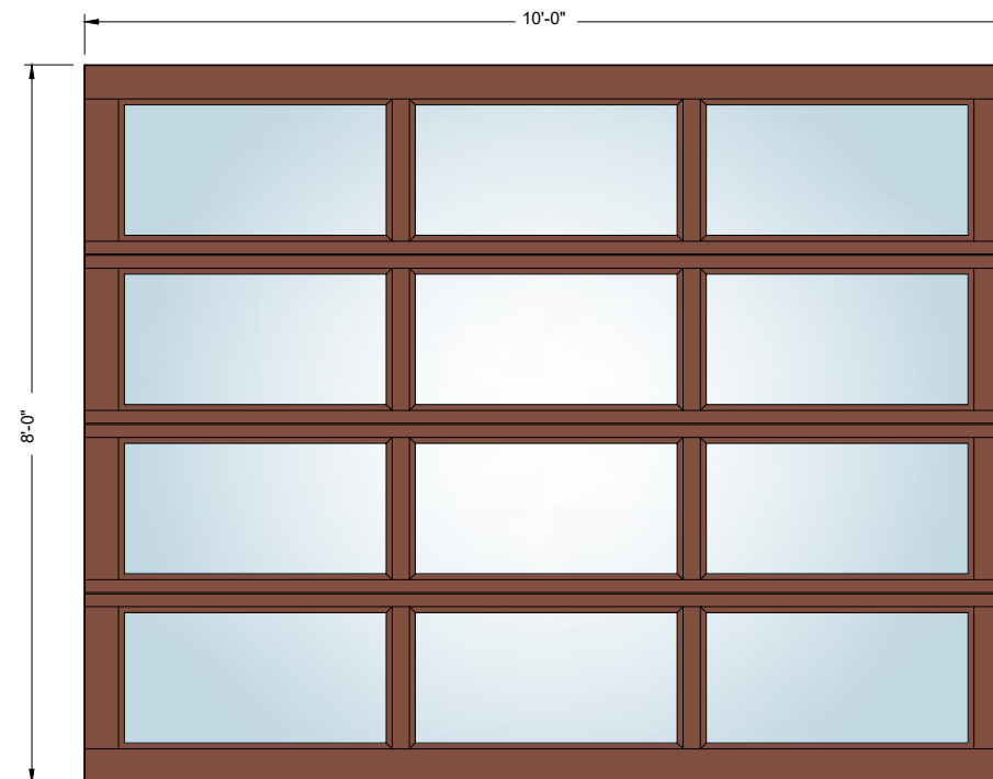
10' x 8' 3-Lite
