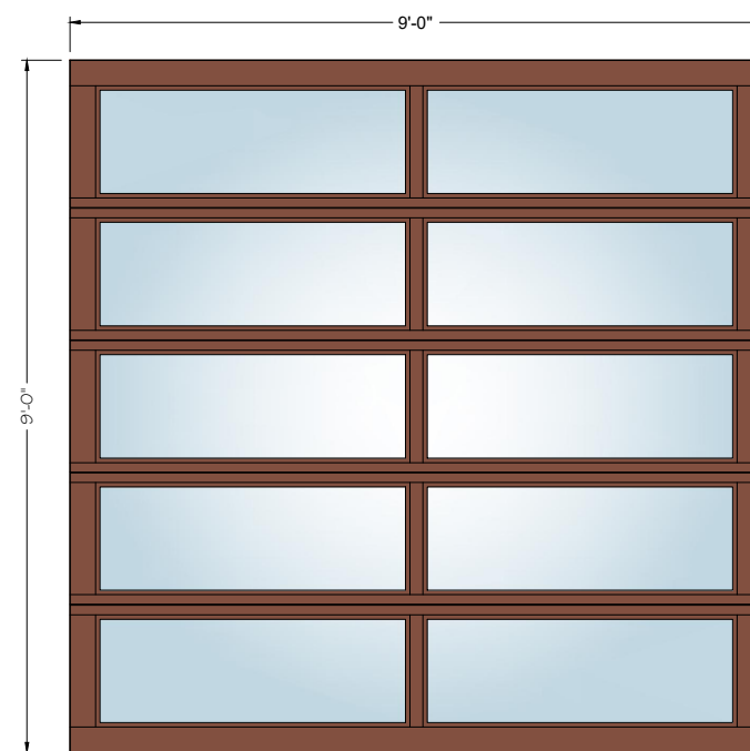
9' x 9' 2-Lite
