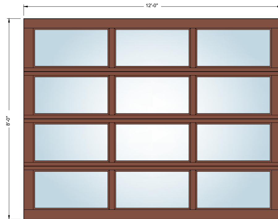
12' x 8' 3-Lite
