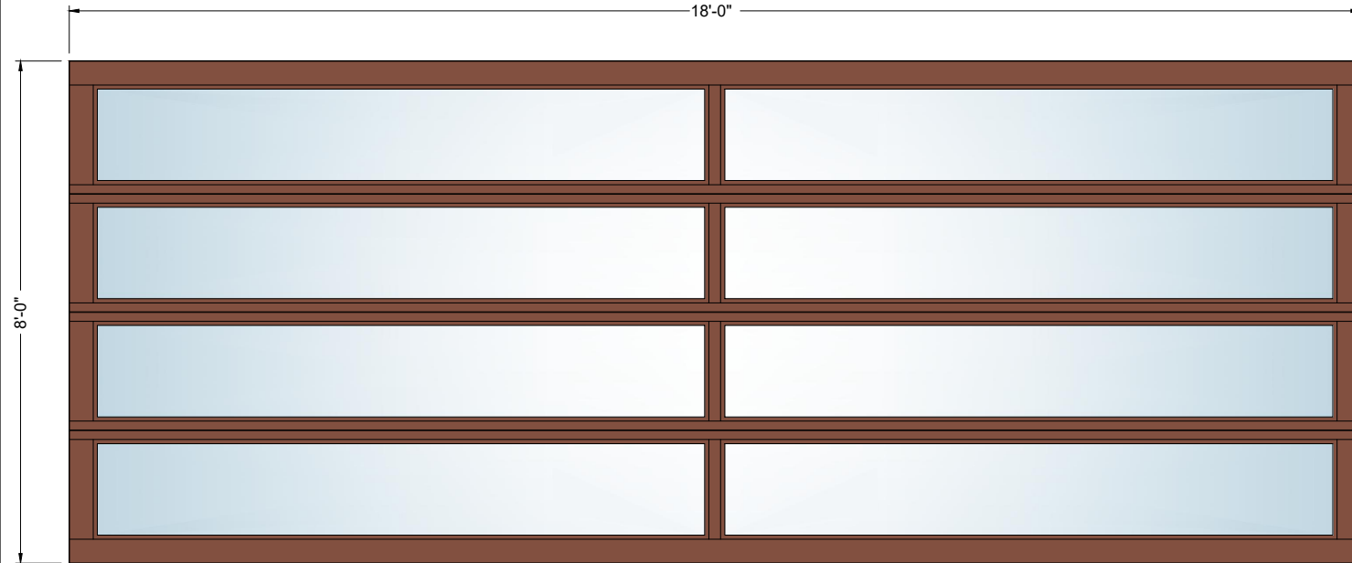
20' x 8' 2-Lite
