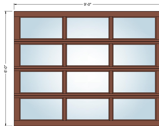
9' x 6' 3-Lite
