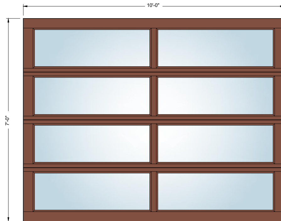
10' x 7' 2-Lite
