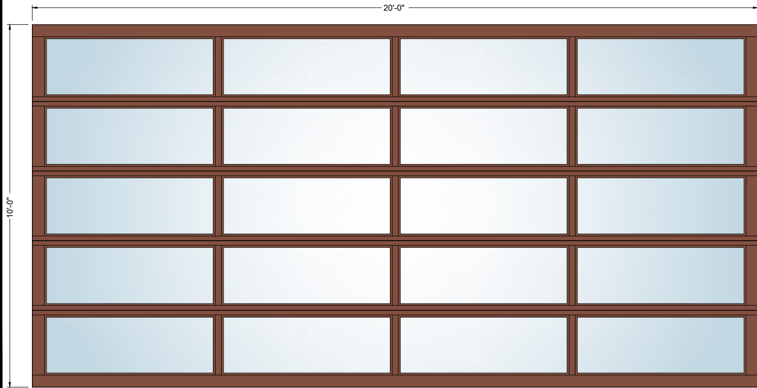
20' x 10' 4-Lite
