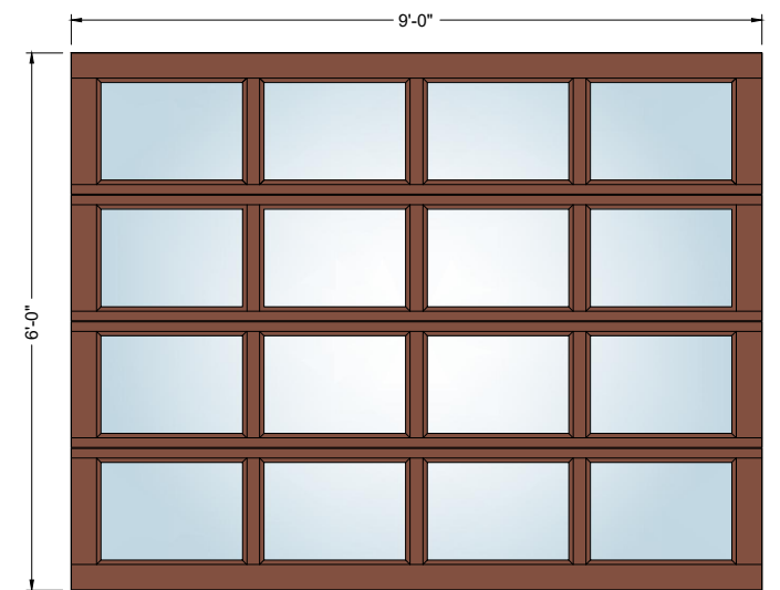
9' x 6' 4-Lite
