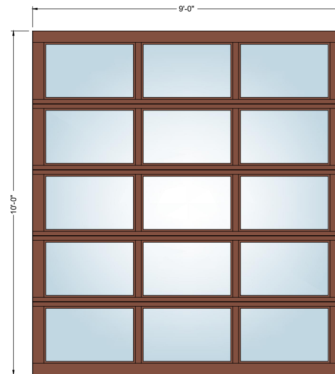
9' x 10' 3-Lite
