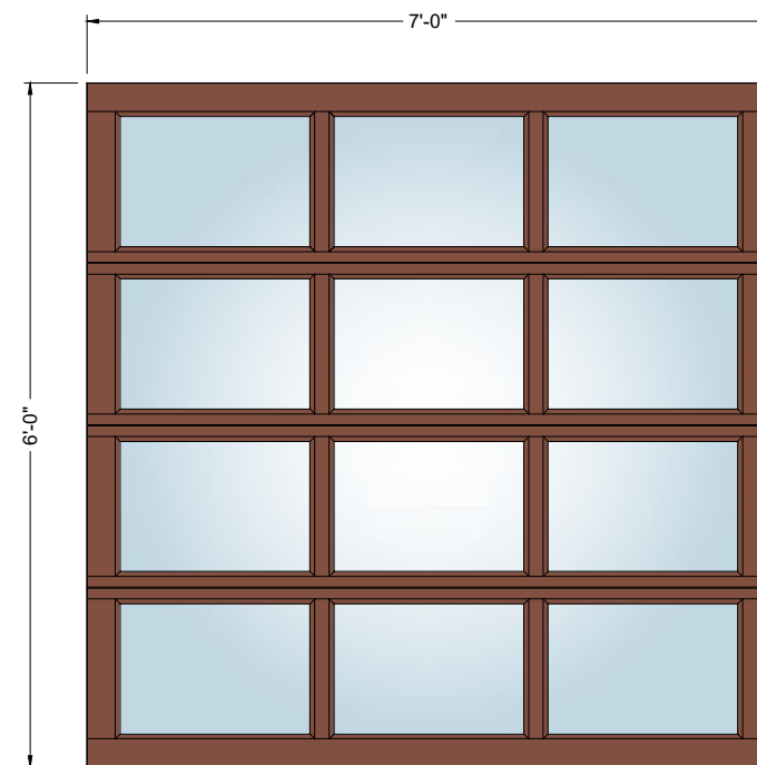
6' x 7' 3-Lite
