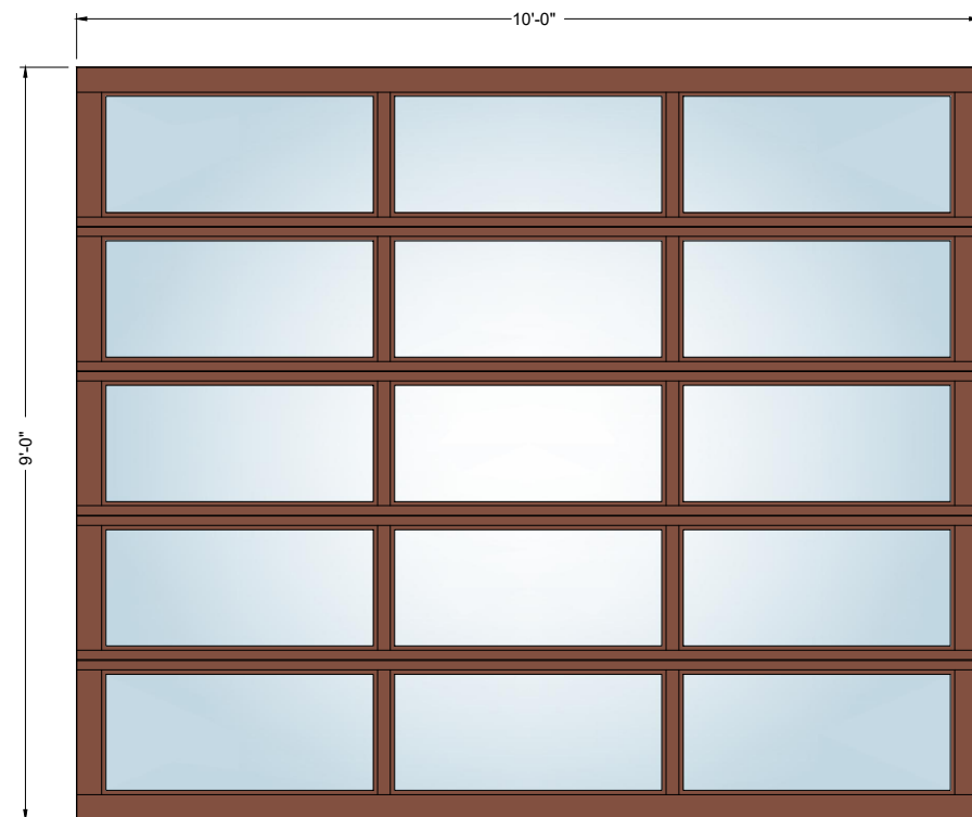
10' x 9' 3-Lite
