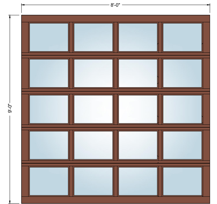
8' x 9' 4-Lite
