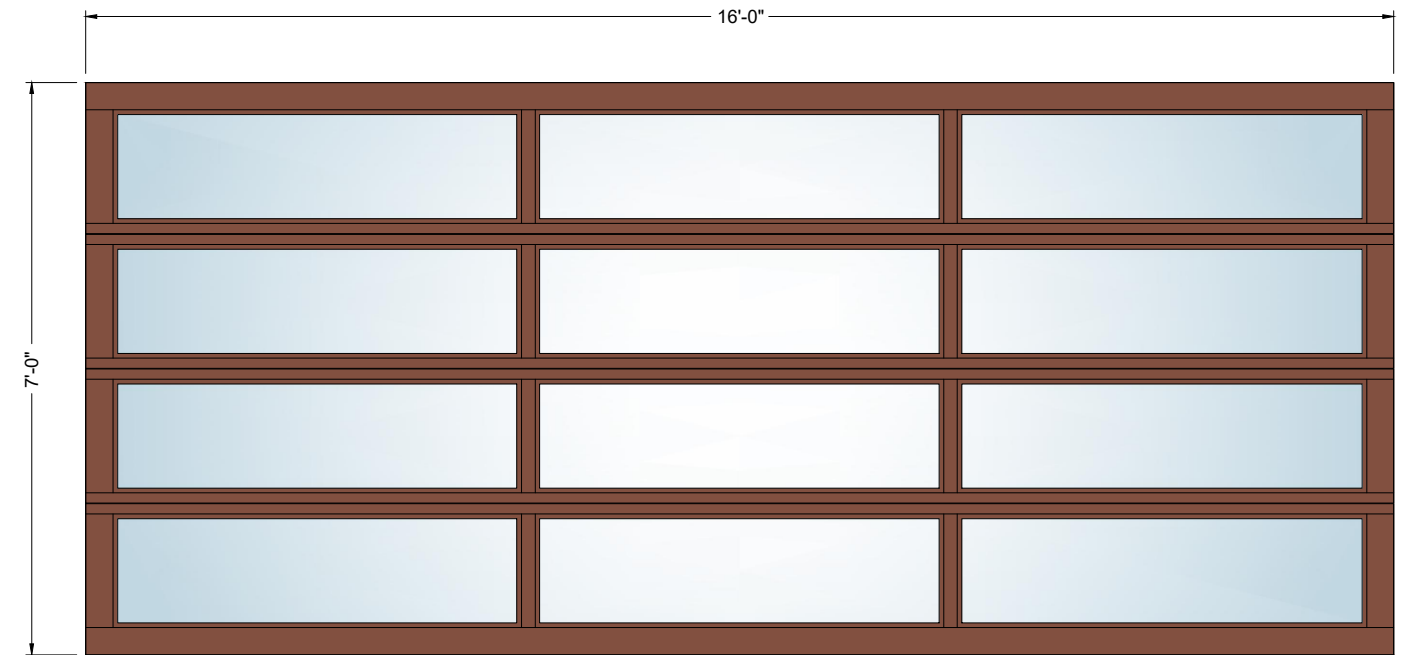
16' X 7' 3-Lite
