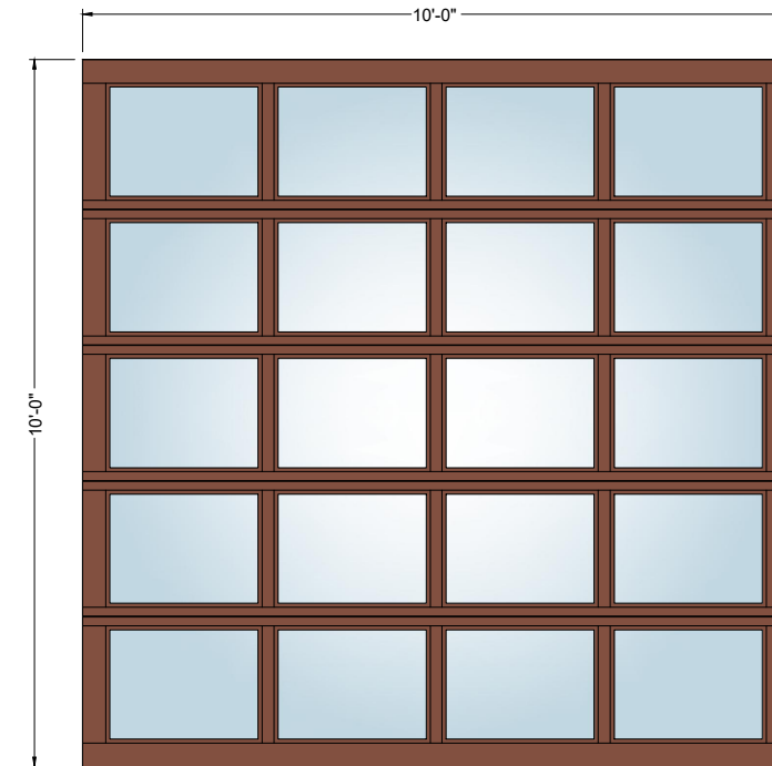
10' x 10' 4-Lite
