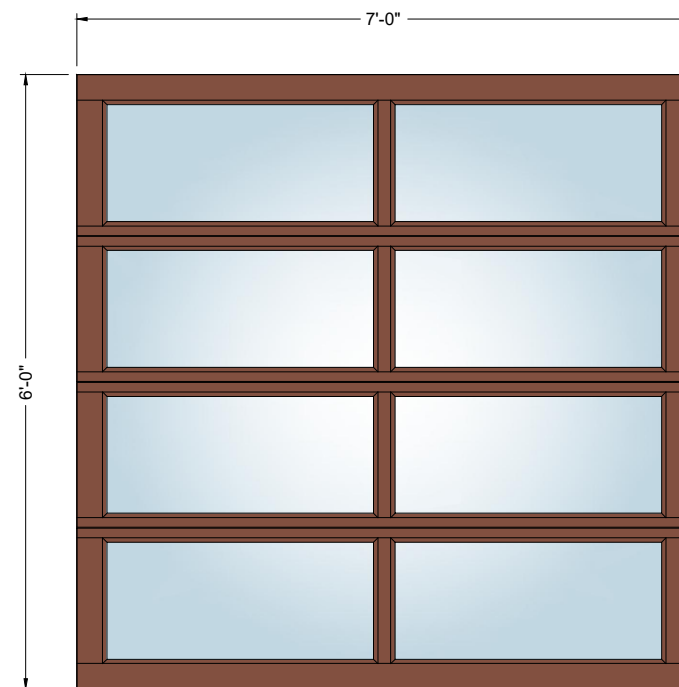
6' x 7' 2-Lite
