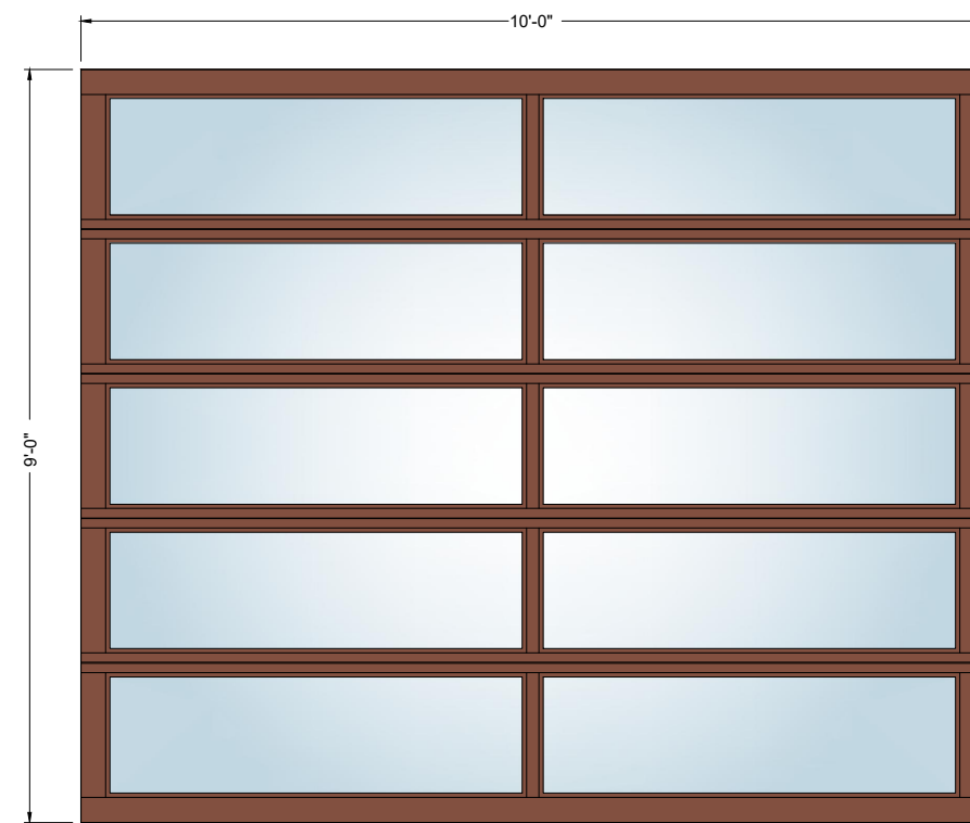
10' x 9' 2-Lite
